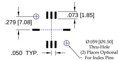
Typical PCB Pad layout
