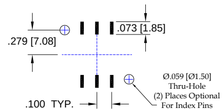
Typical PCB Pad layout
