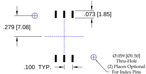
Typical PCB Pad layout
