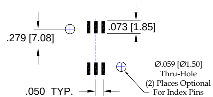
Typical PCB Pad layout
