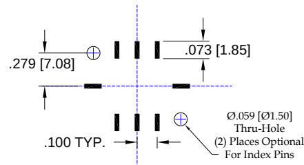
Typical PCB Pad layout
