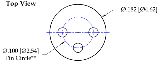
Fig.108 Top View
